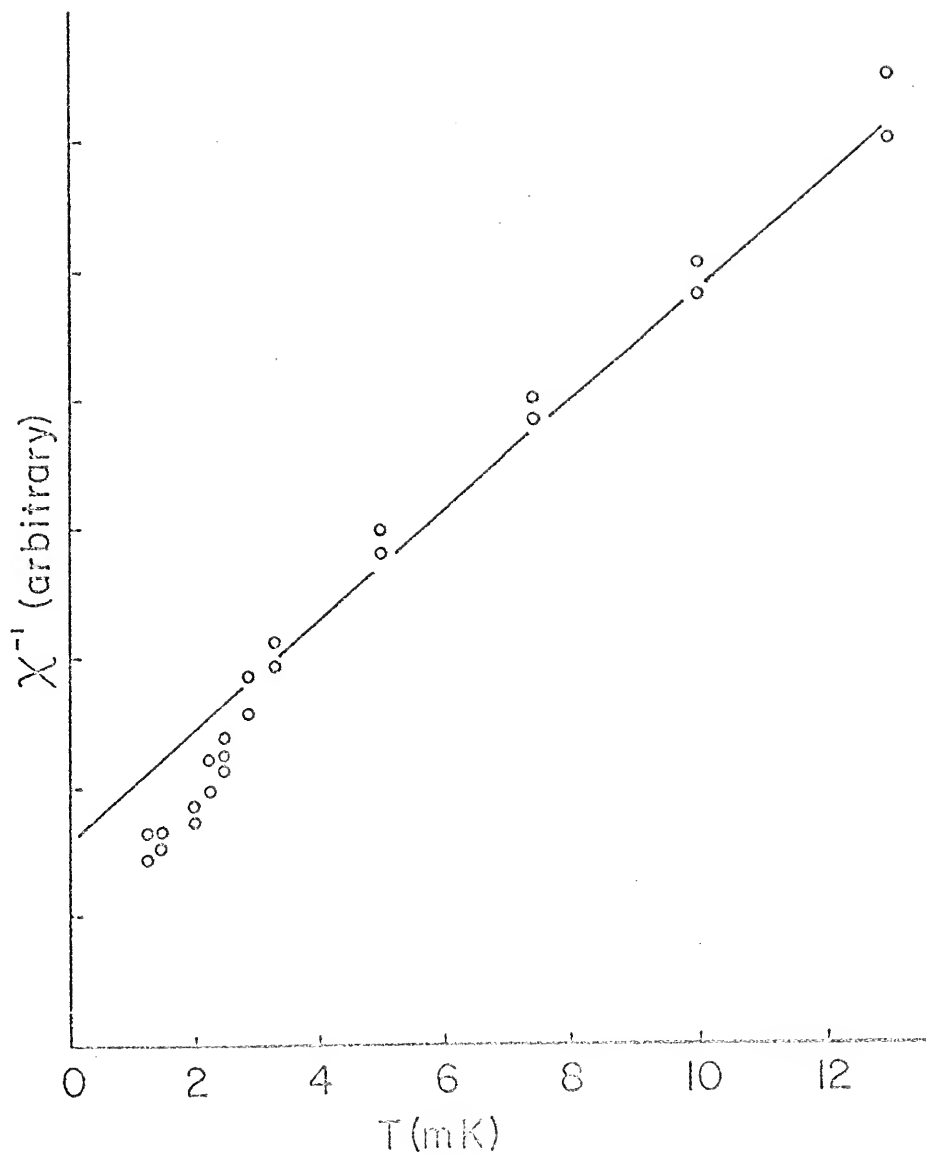
Fig. 12 Curie-Weiss plot of solid Helium three inverse susceptibility.
